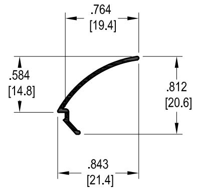
Monolithic Glazing Stop
