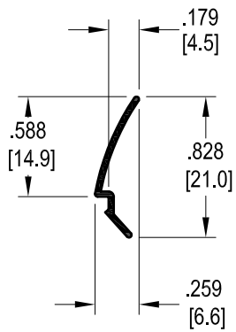
Standard Glazing Stop
