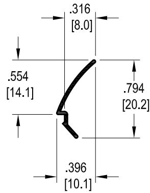
Picture Frame Glazing Stop
