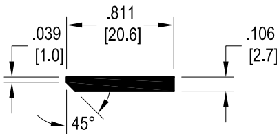
Standard Setting Block
