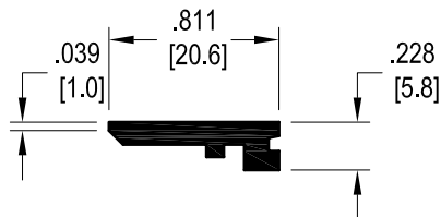
Fixed-Lite Setting Block
