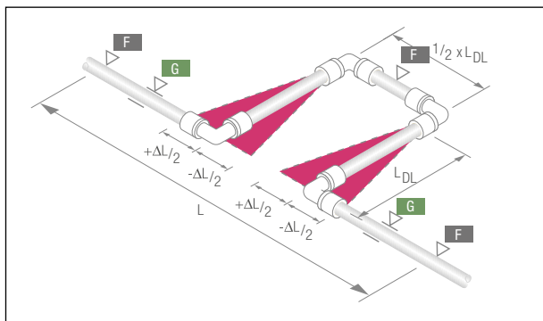
Fig. 6-18 U expansion bends L_{DL} Length of deflection leg \Delta L Thermal length change L Pipe length
