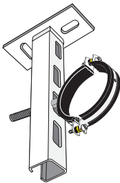
Fixed bracket with Unistrut
