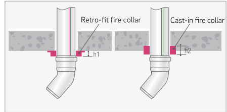
Installation of fireproof collar in ceiling*
