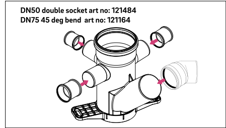
Floor waste gully with double sockets on inlets and 45° bend on outlet
