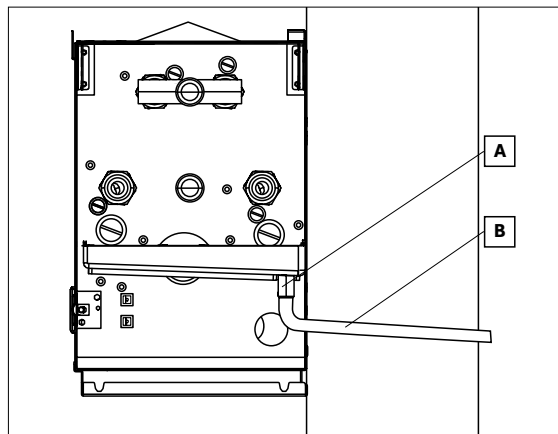
A Drain connection B Drain pipe
