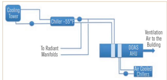
FIGURE 4: Radiant system diagram.
