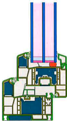
Calculation model
