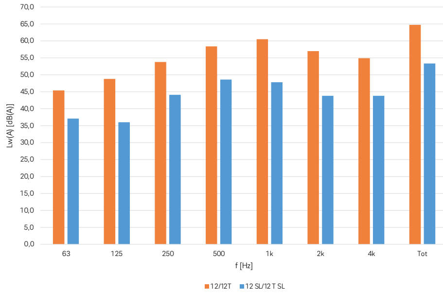
LW(A) Monoblocco Easy Pump 12, 12T Monoblocco Easy Pump SL12/SL12T [dB(A)]
