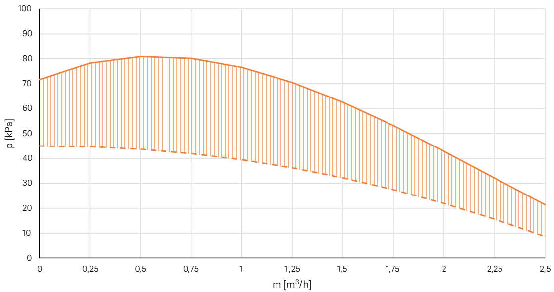
Monoblocco Easy Pump 10, 10T, 12, 12T, SL12, SL12T
