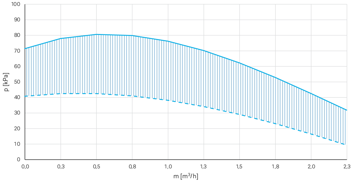
Monoblocco Easy Pump 04, 06, 08, SL08
