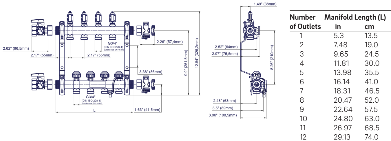
Fig. 1: Manifold dimensions
