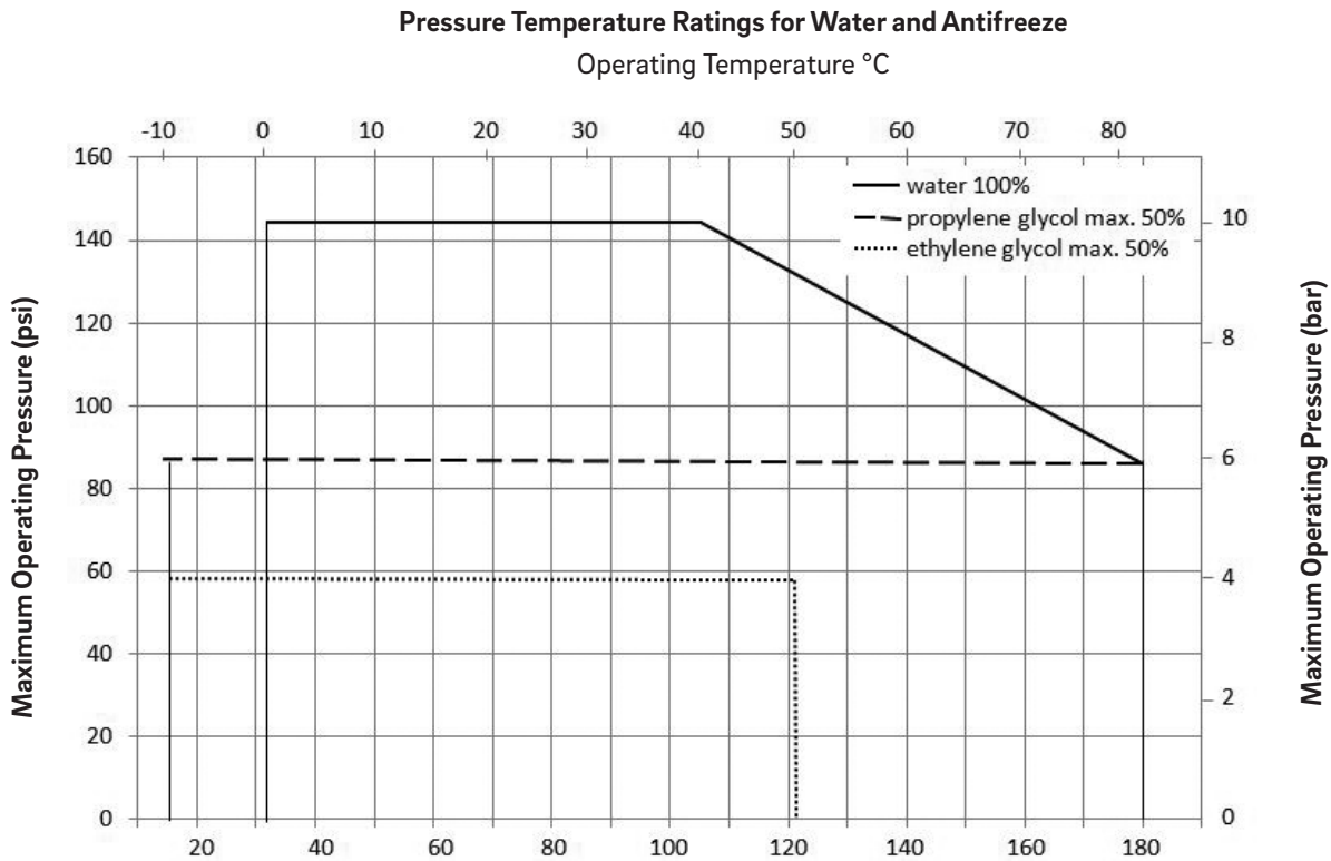
Fig. 2: Manifold temperature and pressure capabilities for different system fluids Note: Operating temperature and pressure must stay below corresponding line for appropriate fluid type.
