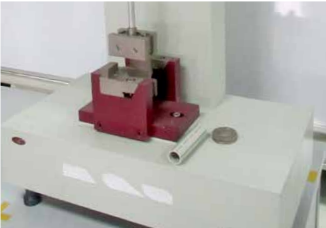
Fig. 3-4 Impact resistance test apparatus
