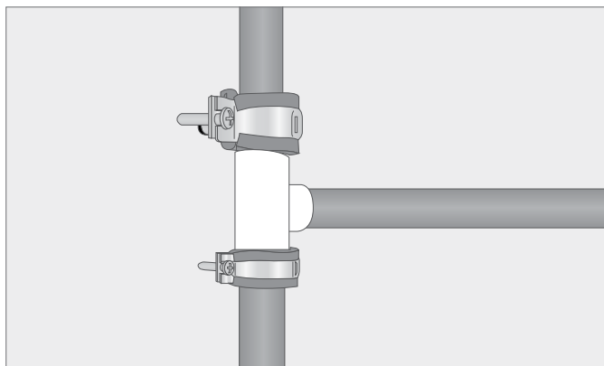
Fig. 11-1 Anchor point made by pipe clamps
