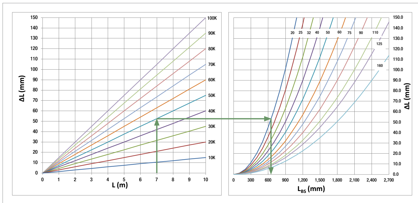
Fig.13-3 Linear expansion and deflection leg length of RAUFUSION PP-R pipes size 20 - 125 mm
