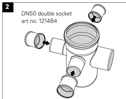
Floor waste gully with double sockets on inlets
