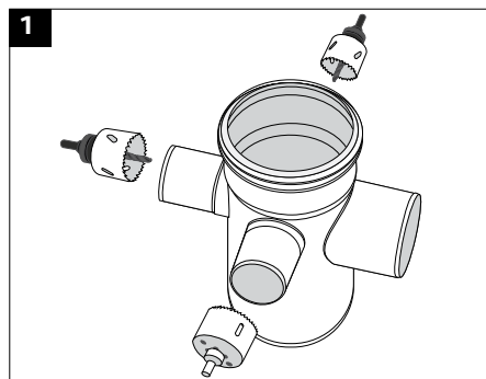
Floor waste gully art. no. 100391-001
