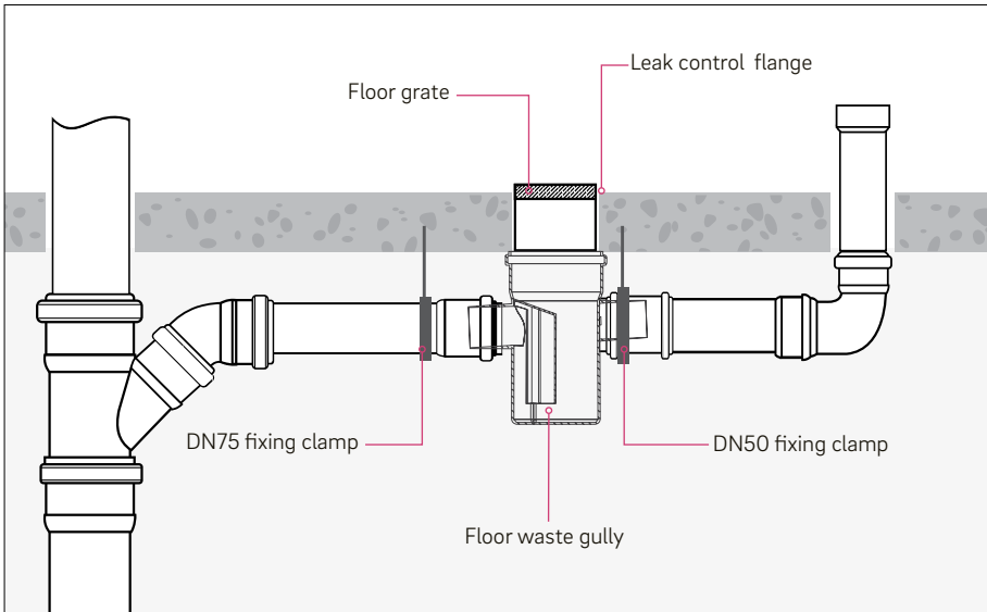
Shower gully - Bracketing*
