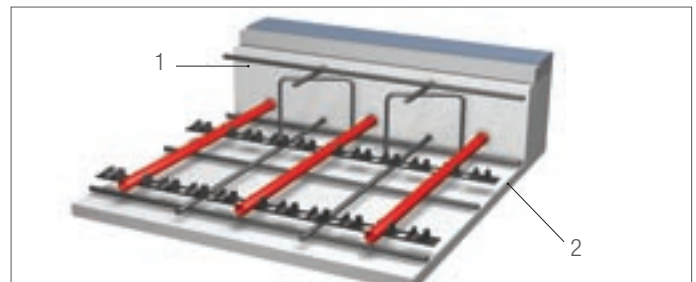
Diagram 3 - Floor panel reinforced with steel fibres; special construction heating pipes assembled to the clamping rails. 1 Concrete plate 2 Foundation
