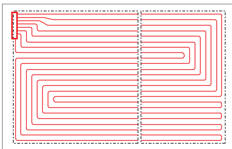
Heating circuits run in parallel (zone formation)
