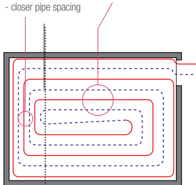
Compressed Perimeter Zone with reverse spiral pattern
