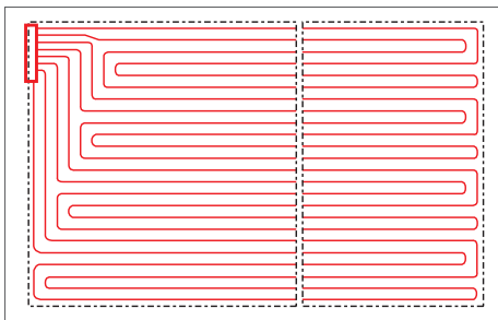
Heating circuits separate
