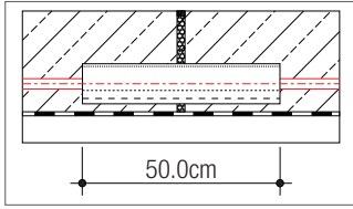
Un-doweled expansion joint with protection via 100 % insulating tube
