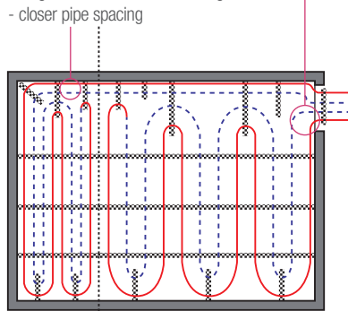
Separate Perimeter Zone with double meander pattern
