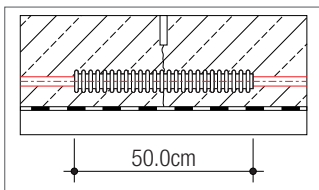
Dummy joint, pressed joint with REHAU protective sleeve
