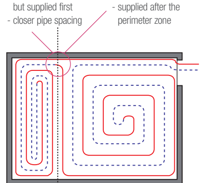
Upstream Perimeter Zone with reverse spiral pattern
