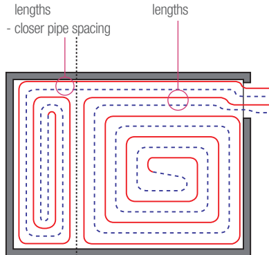
Separate Perimeter Zone with reverse spiral pattern
