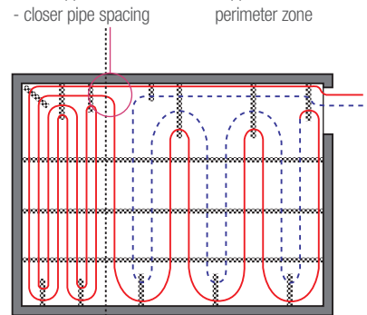
Upstream Perimeter Zone with double meander pattern
