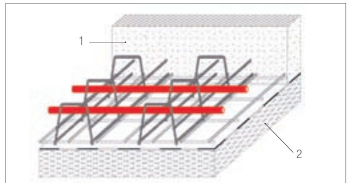
Diagram 2 - Floor panel reinforced with steel grids; special construction heating pipes assembled at the centre of the plate. 1 Concrete plate 2 Foundation
