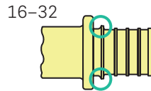
Fig. 36-4 Fitting with fully formed pre-stop, size 16–32
