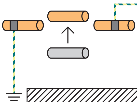
Fig. 35-12 Earth bonding when exchanging pipes
