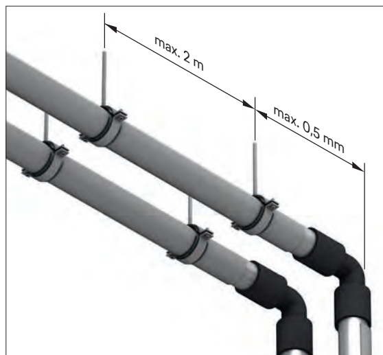
Fig. 31-3 Maximum pipe clamp intervals
