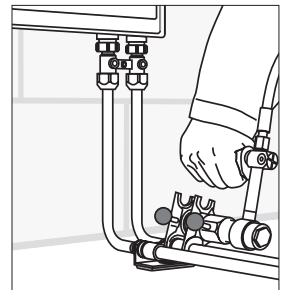
Fig. 14-11 Create compression sleeve connection
