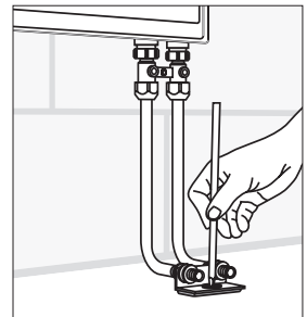
Fig. 14-9 Mark the fixing point
