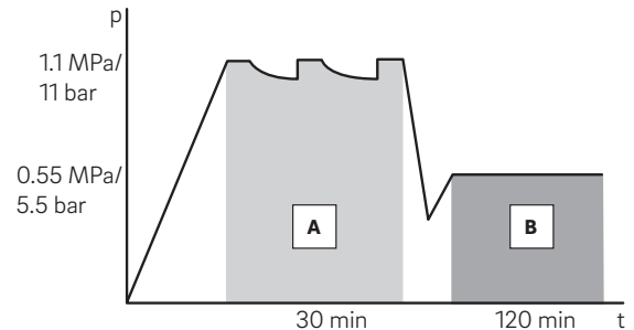
Fig. 08-2 Pressure test based on ZVSHK-information sheet for RAUTITAN flex
