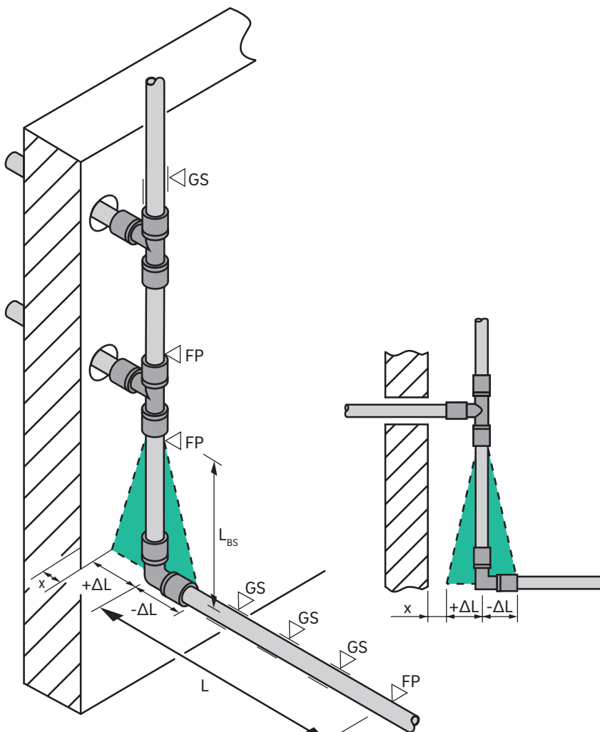
Fig. 34-1 Deflection legs
