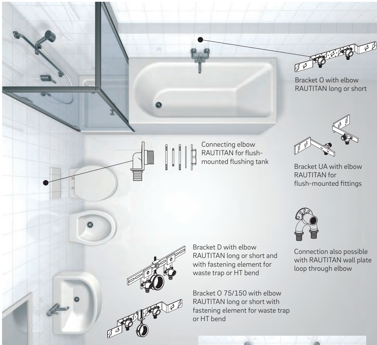
Fig. 06-6 Bracket range in the bathroom and WC
