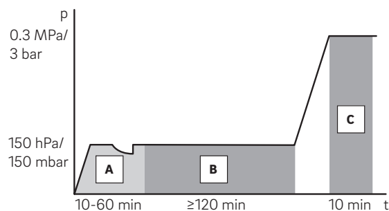
Fig. 08-3 Pressure test for pressure test with compressed air or inert gas
