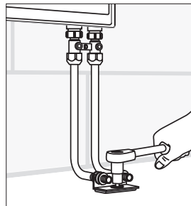
Fig. 14-10 Screw the fixing unit to the floor
