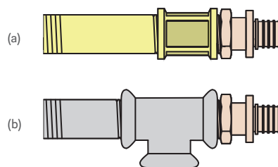
Fig. 25-10 Adapter with RAUTITAN male thread screwed into: (a) Brass fittings (b) Systems with galvanised pipes and fittings
