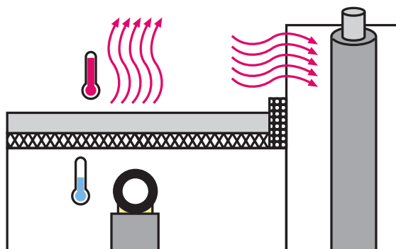
Fig. 35-5 Laying under hot asphalt screed
