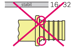
Fig. 36-3 Brass fitting with partially formed pre-stop, size 16–32
