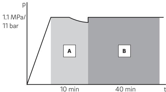
Fig. 08-1 Pressure test based on ZVSHK-information sheet for RAUTITAN stabil
