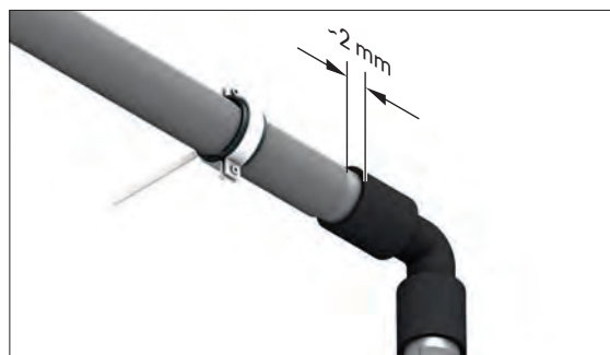
Fig. 31-2 Let the pipe support channel end approx. 2 mm before the compression sleeve
