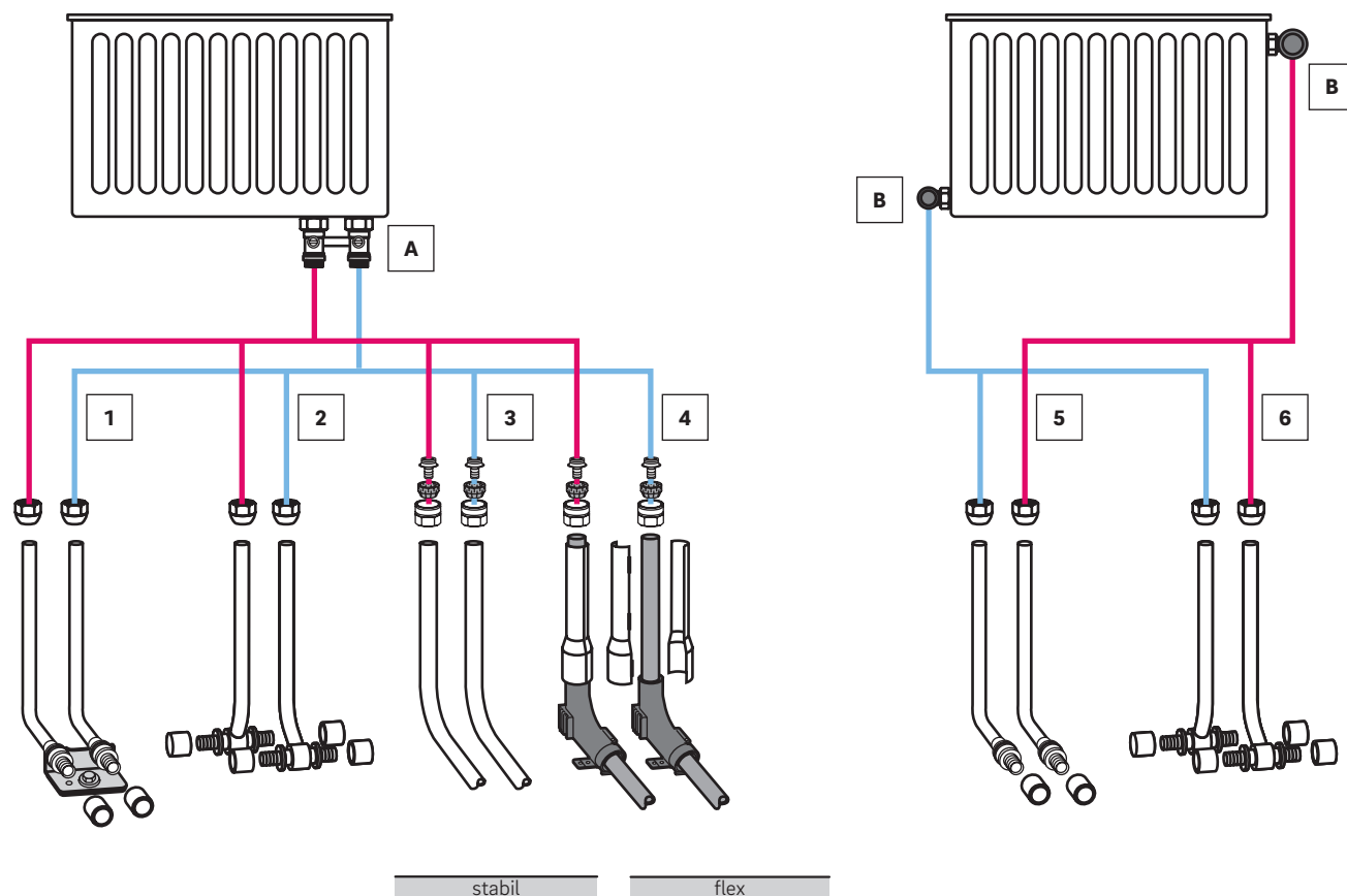
Fig. 12-1 Overview: Radiator connection from the floor
