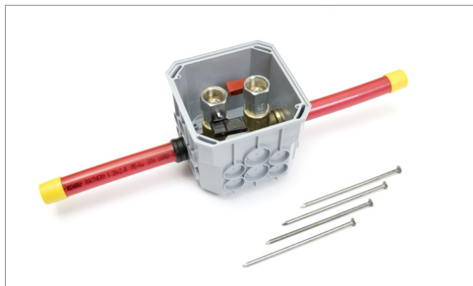
Fig. 2-14 CCT extension box
