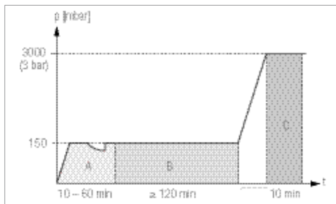
Fig. 3-1 Pressure test diagram for pressure tests with oil-free compressed air/ inert gas
