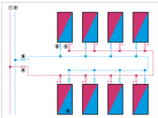
Fig. 2-10 Schematic illustration of a two-line system
