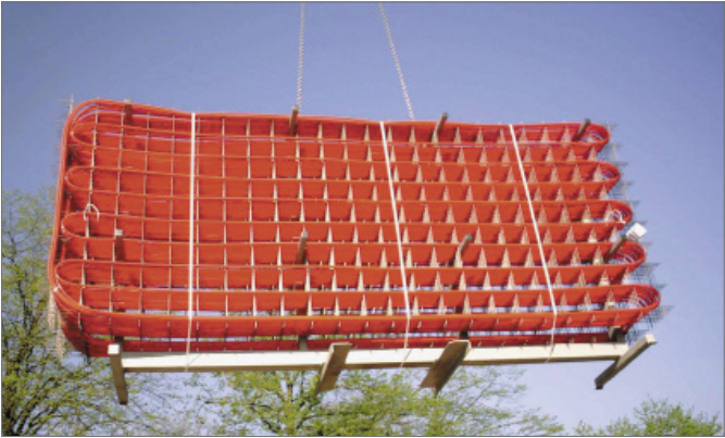
Fig. 2-24 REHAU CCT transport frame
